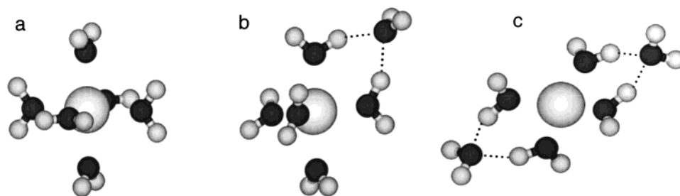
Figure 5. Representative geometries for the (a) Mg^{2+}(H_2O)_6 , (b) Mg^{2+}(H_2O)_5(H_2O) , and (c) Mg^{2+}(H_2O)_4(H_2O)_2 structures. Hydrogen bonds are indicated with dashed lines.
