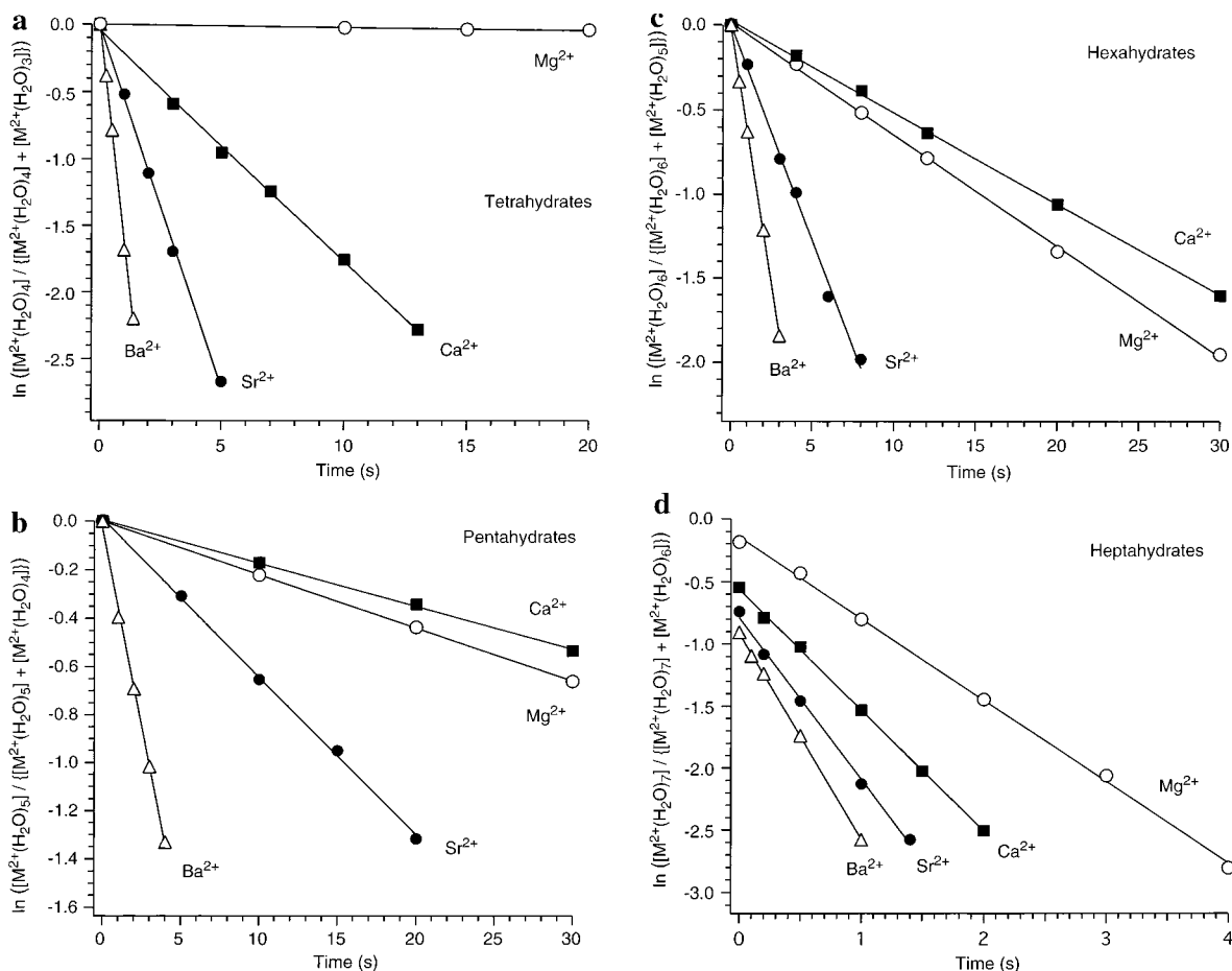
Figure 6. Collisional activated dissociation data for (a) M^{2+}(H_2O)_4 , (b) M^{2+}(H_2O)_5 , (c) M^{2+}(H_2O)_6 , and (d) M^{2+}(H_2O)_7 clusters. M = magnesium (○), calcium (■), strontium (●), and barium (△). Average center-of-mass energies and average collision frequencies are given in Table 2.
